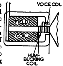
Location of hum-bucking coil in an electrodynamic loudspeaker.
